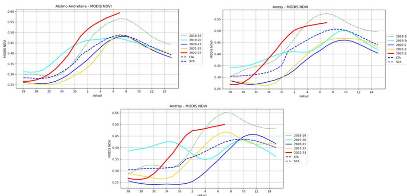
Fig.3 Comparaison profil NDVI 2018/2019/2020/2021/2022
